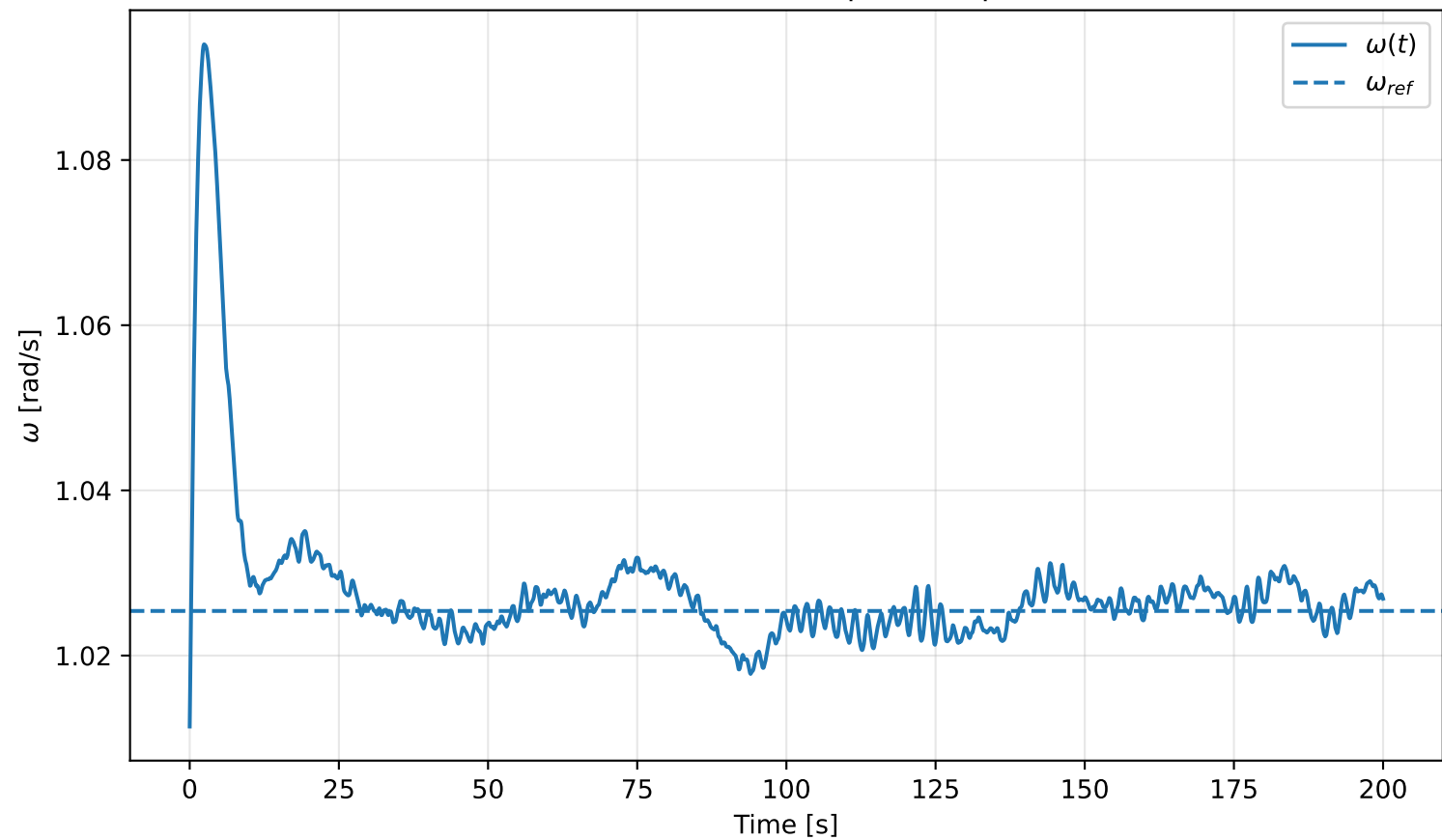
Turbulent wind: rotor-speed response
